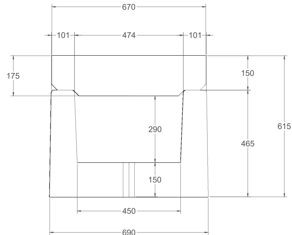
SECTION VIEW
