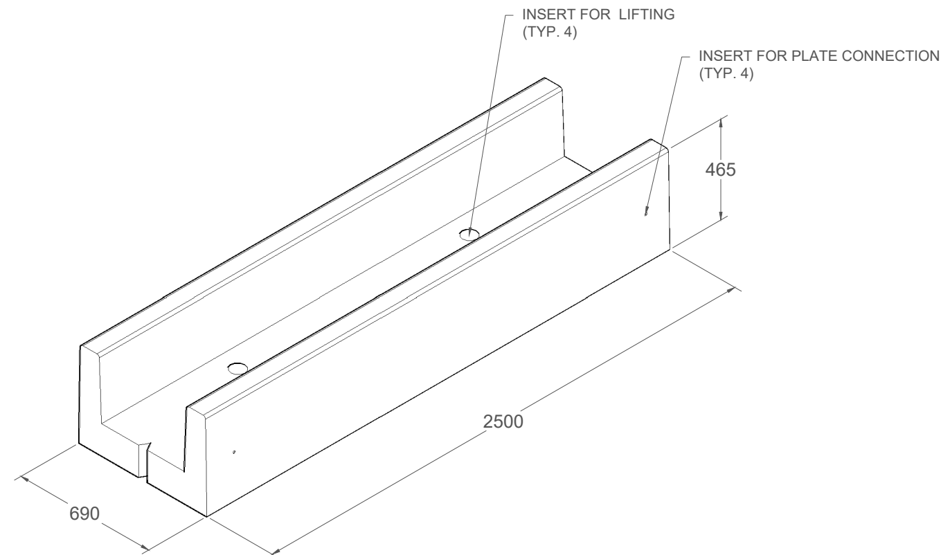
ISOMETRIC VIEW TROUGH 2500mm x 690mm x 465mm 1030 KG
